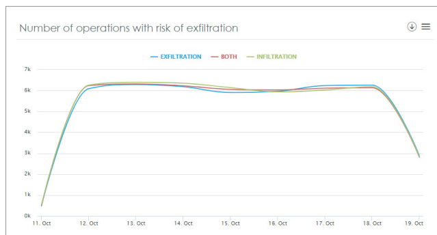
Figure 1 - This information enables organizations to monitor and determine the usual number of exfiltration operations, detecting deviations caused by security incidents.
